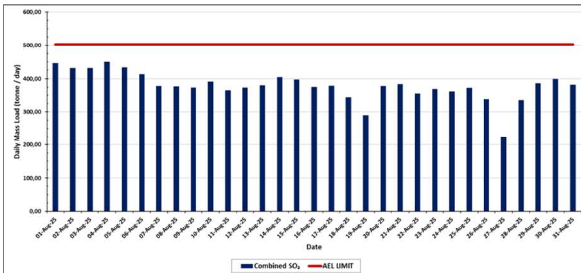
Figure 6: SO daily average SO 2 load-based limit for the period 1 st August 2025 to 31 st August 2025
