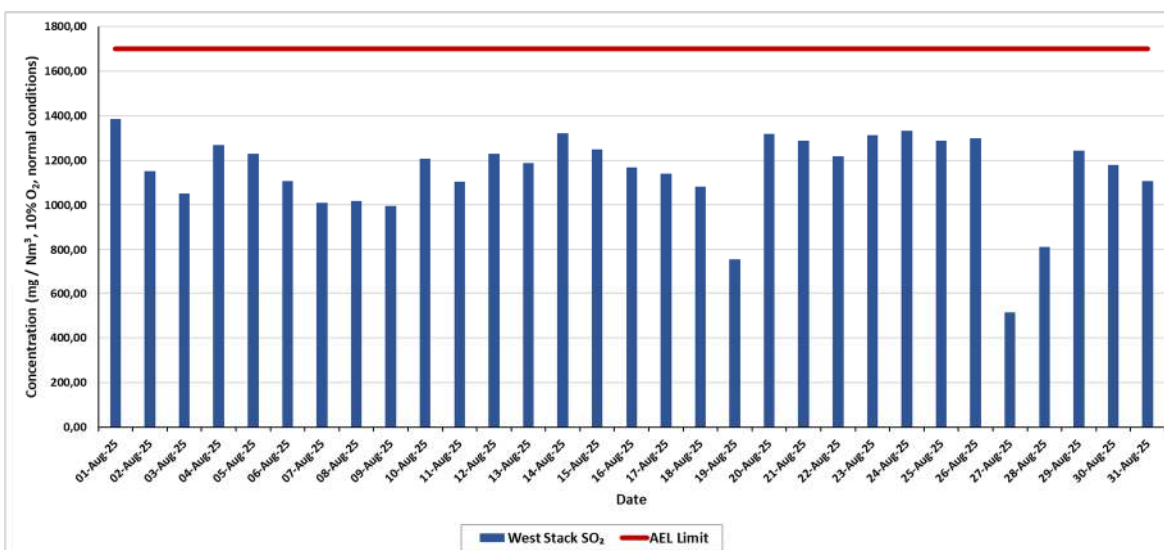
Figure 5: SO measured daily average SO 2 emissions in the West stack at 10% O 2 correction for the period 1 st August 2025 to 31 st August 2025
