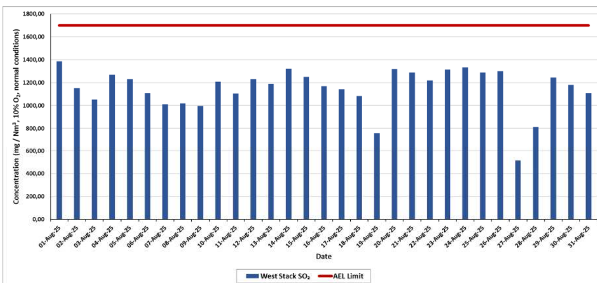
Figure iii: SO measured daily average SO 2 emissions in the West stack at 10% O 2 correction for the period 1 st August to 31 st August 2025
