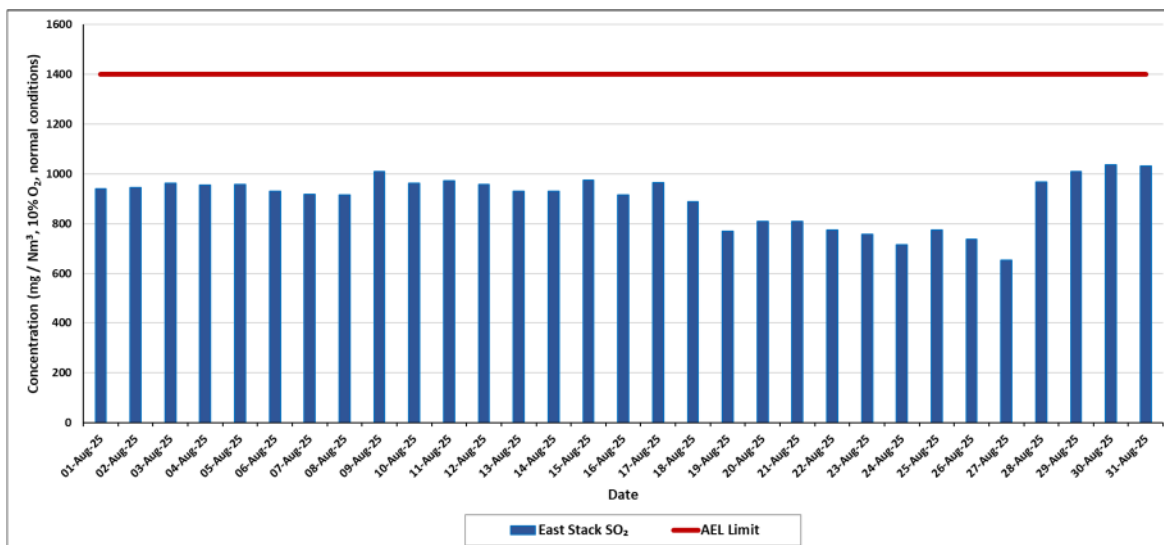
Figure 4: SO measured daily average SO 2 emissions in the East stack at 10% O 2 correction for the period 1 st August 2025 to 31 st August 2025
