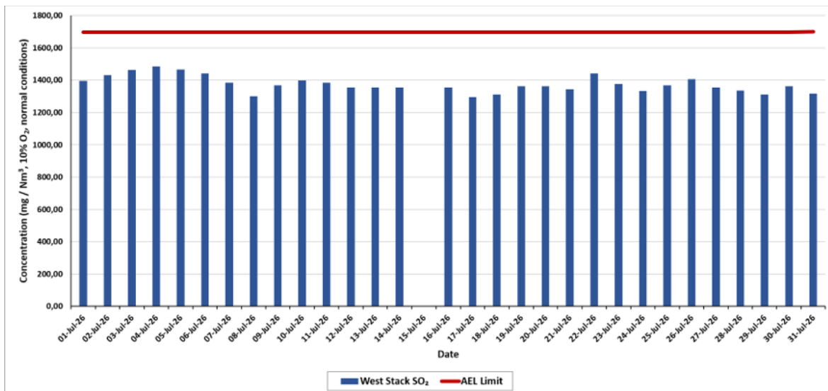
Figure 5: SO measured daily average SO 2 emissions in the West stack at 10% O 2 correction for the period 1 st July 2026 to 31 st July 2026 1
