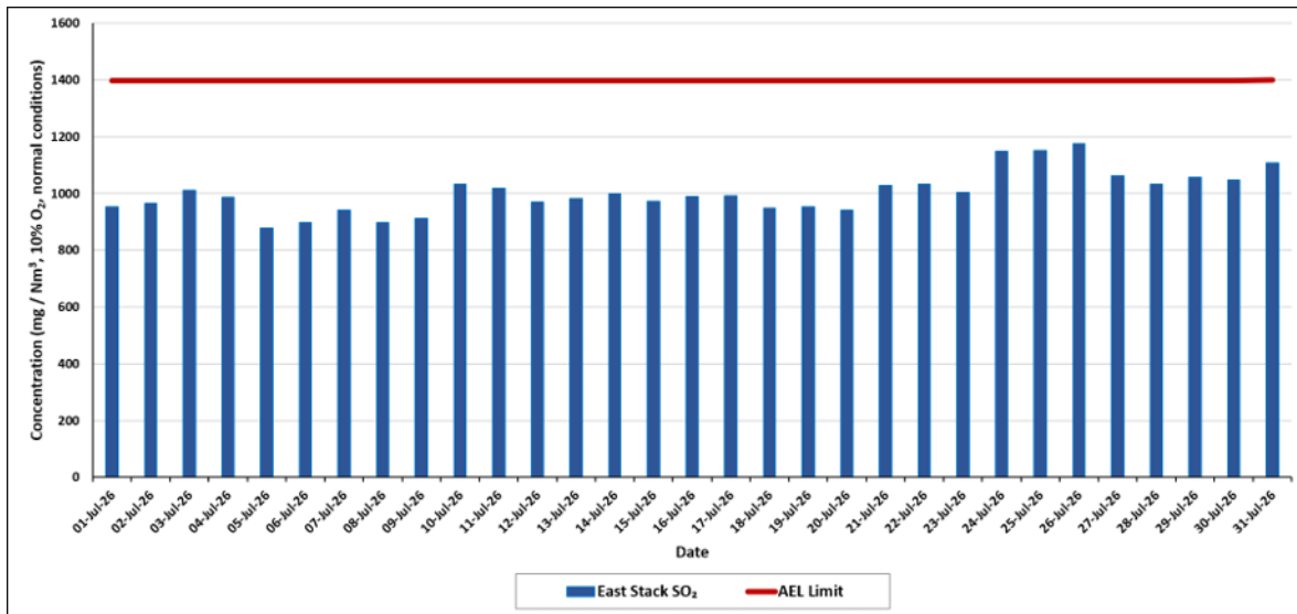
Figure 4: SO measured daily average SO 2 emissions in the East stack at 10% O 2 correction for the period 1 st July 2026 to 31 st July 2026
