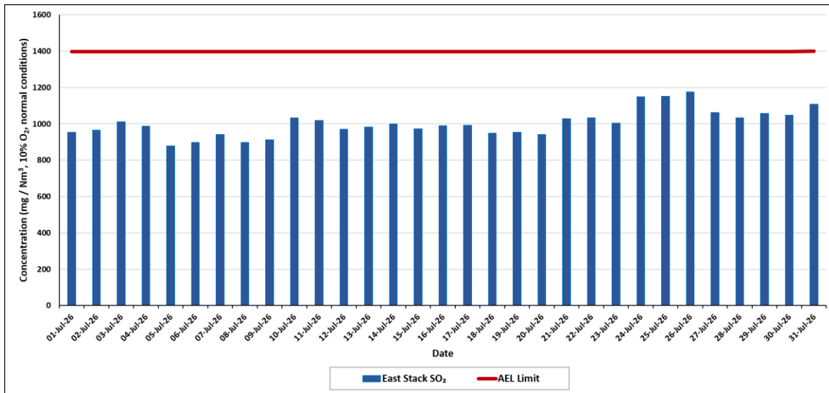
Figure ii: SO measured daily average SO 2 emissions in the East Stack at 10% O 2 correction for the period 1 st July to 31 st July 2026
