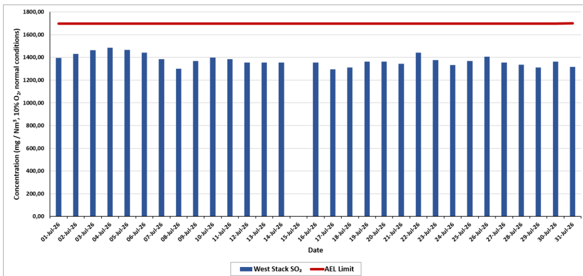
Figure iii: SO measured daily average SO 2 emissions in the West Stack at 10% O 2 correction for the period 1 st July to 31 st July 2026 1
