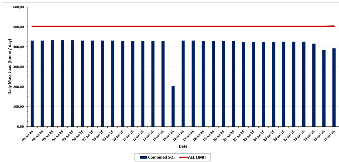
Figure iv: SO monthly average SO 2 load-based limit for the period 1 st July to 31 st July 2026 1
