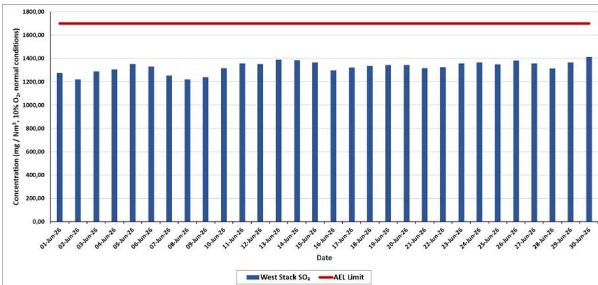
Figure 5: SO measured daily average SO 2 emissions in the West stack at 10% O 2 correction for the period 1 st June 2026 to 30 th June 2026
