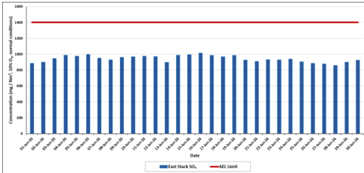
Figure ii: SO measured daily average SO 2 emissions in the East Stack at 10% O 2 correction for the period 1 st June to 30 th June 2026
