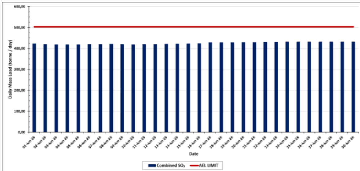
Figure 6: SO monthly average SO 2 load-based limit for the period 1 st June 2026 to 30 th June 2026
