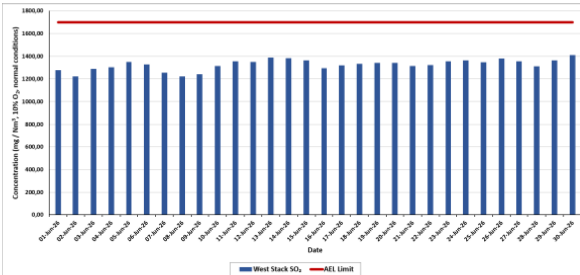
Figure iii: SO measured daily average SO 2 emissions in the West Stack at 10% O 2 correction for the period 1 st June to 30 th June 2026
