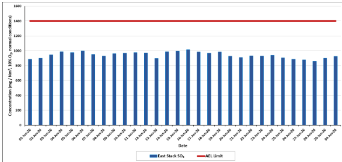
Figure 4: SO measured daily average SO 2 emissions in the East stack at 10% O 2 correction for the period 1 st June 2026 to 30 th June 2026
