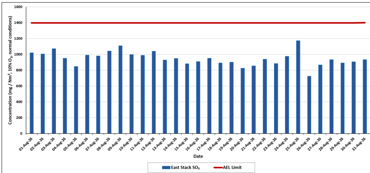
Figure ii: SO measured daily average SO 2 emissions in the East Stack at 10% O 2 correction for the period 1 st August to 31 st August 2026 1
