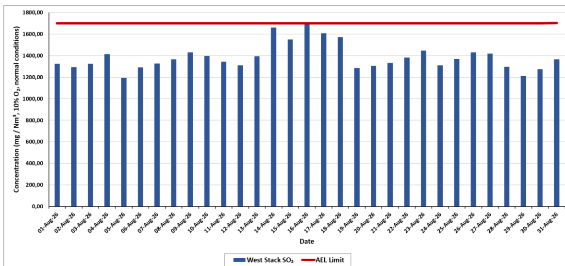
Figure iii: SO measured daily average SO 2 emissions in the West Stack at 10% O 2 correction for the period 1 st August to 31 st August 2026 2 3
