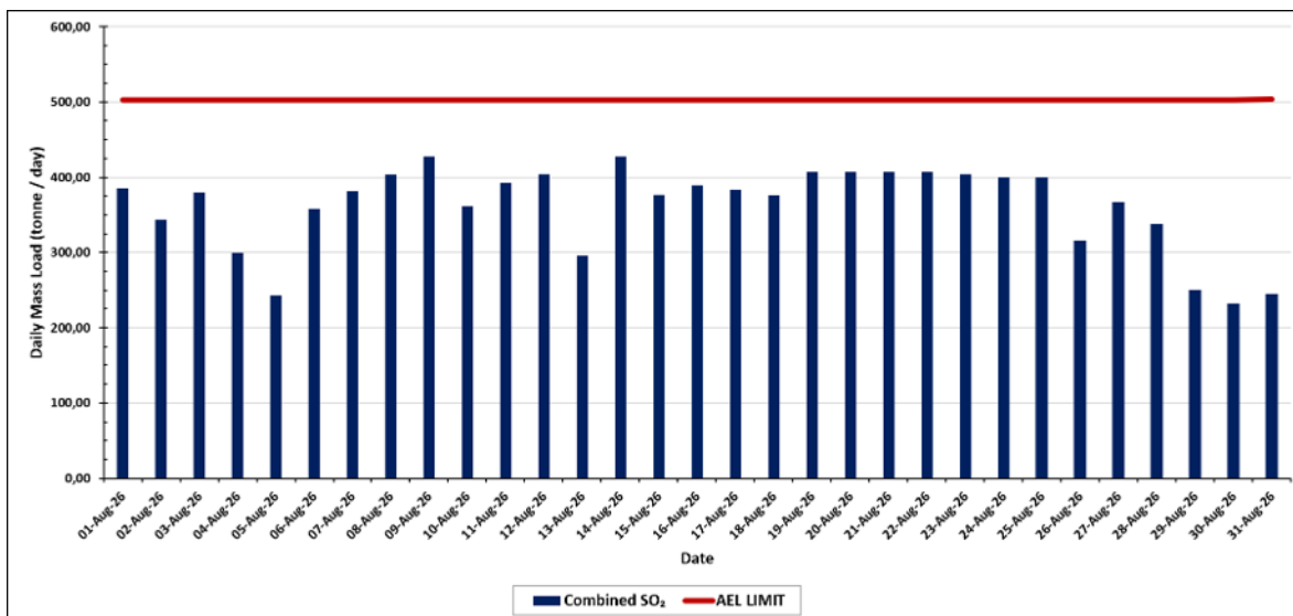
Figure 6: SO monthly average SO 2 load-based limit for the period 1 st August 2026 to 31 st August 2026 4 5
