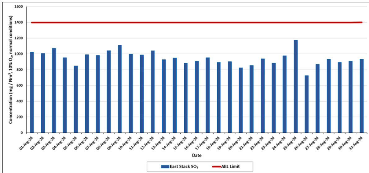
Figure 4: SO measured daily average SO 2 emissions in the East stack at 10% O 2 correction for the period 1 st August 2026 to 31 st August 2026 1
