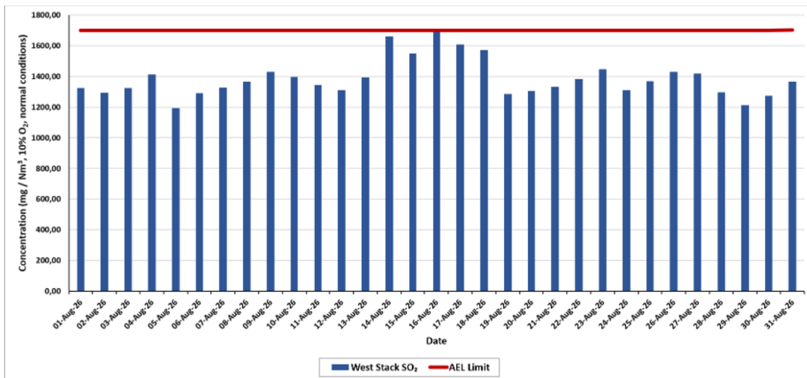
Figure 5: SO measured daily average SO 2 emissions in the West stack at 10% O 2 correction for the period 1 st August 2026 to 31 st August 2026 2 3
